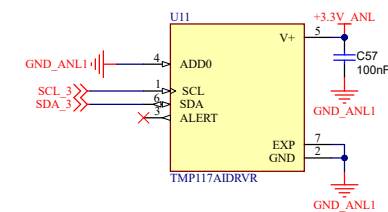
Temperature and Humidity Sensing TMP117 (I2C Address: 0x48)
