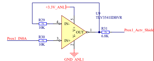
Active Shielding for C-type Electrode
